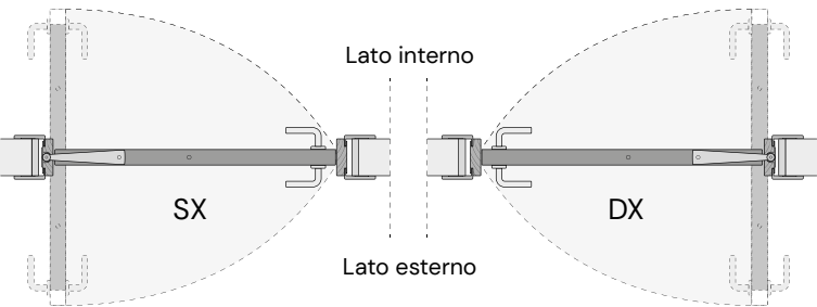
Apertura porta rototraslante Rototranslating opening – Ouverture rotative
